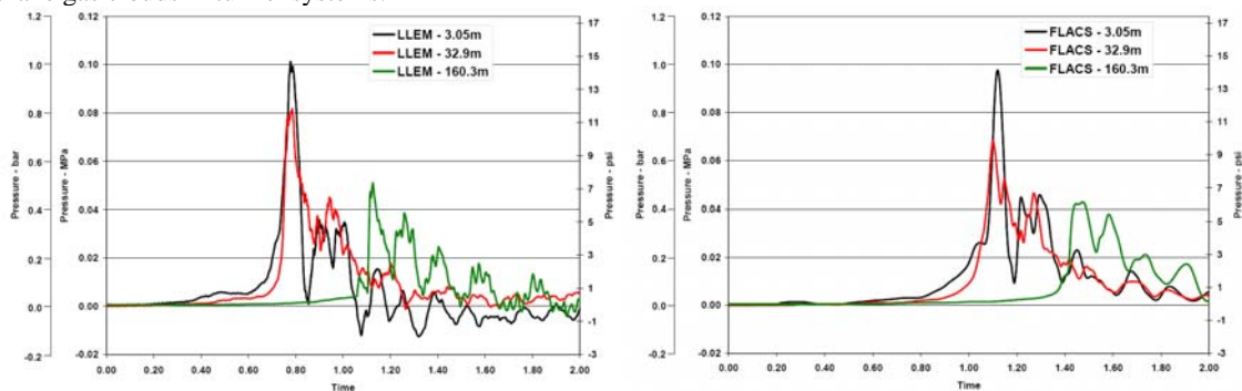
Figure 4. Comparison of FLACS blindly predicted pressures (right plot) and NIOSH test results from Lake Lynn Experimental mines (left plot) for three different locations [9]. The deviation in arrival time is a consequence of the strong ignition source used in the tests.
