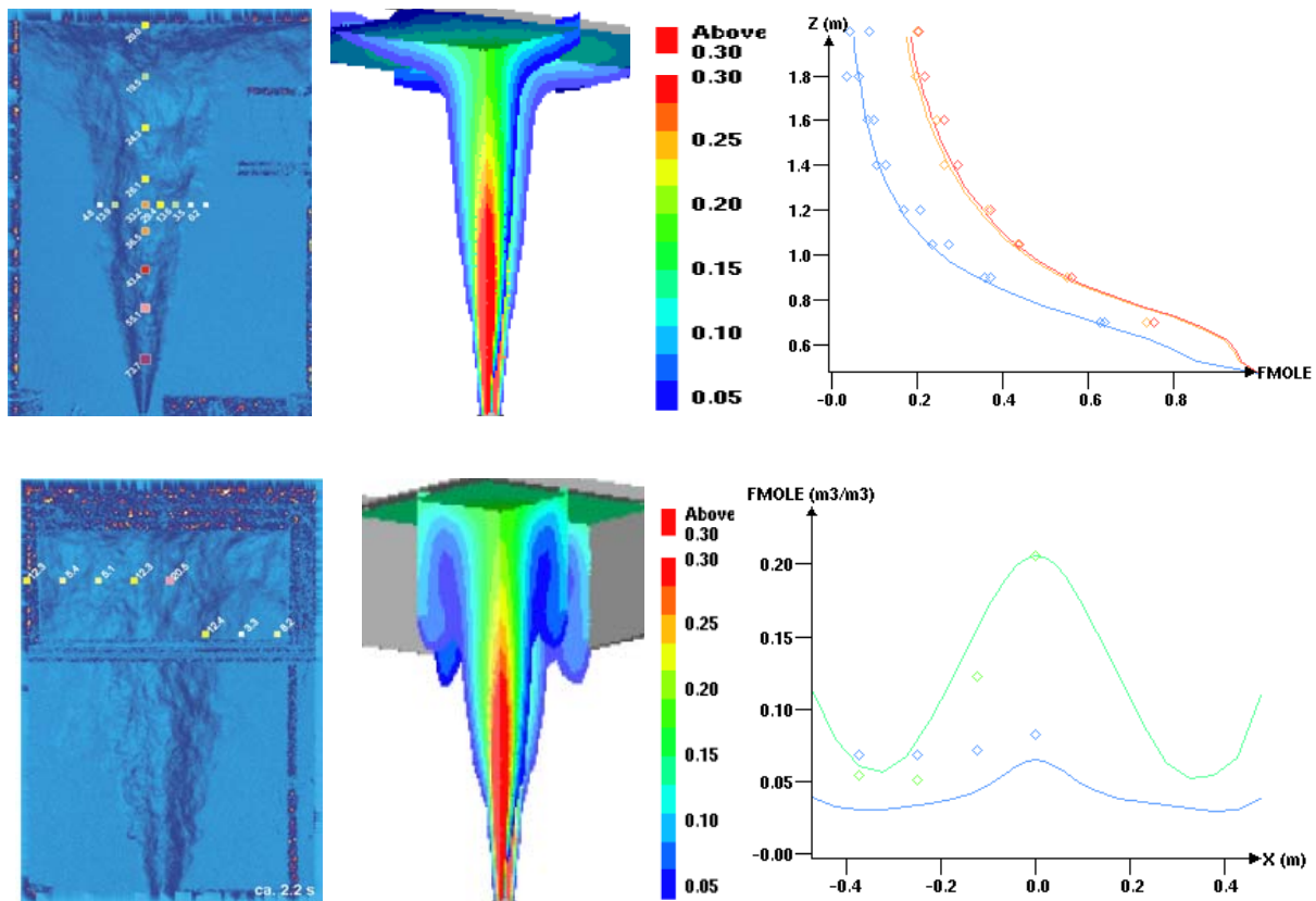
Figure 5. Comparison of experimental photograph/recording with FLACS predicted plume shape and concentrations for release from 21 mm nozzle (3 g/s) in the plate geometry (top) and hood geometry (bottom).
