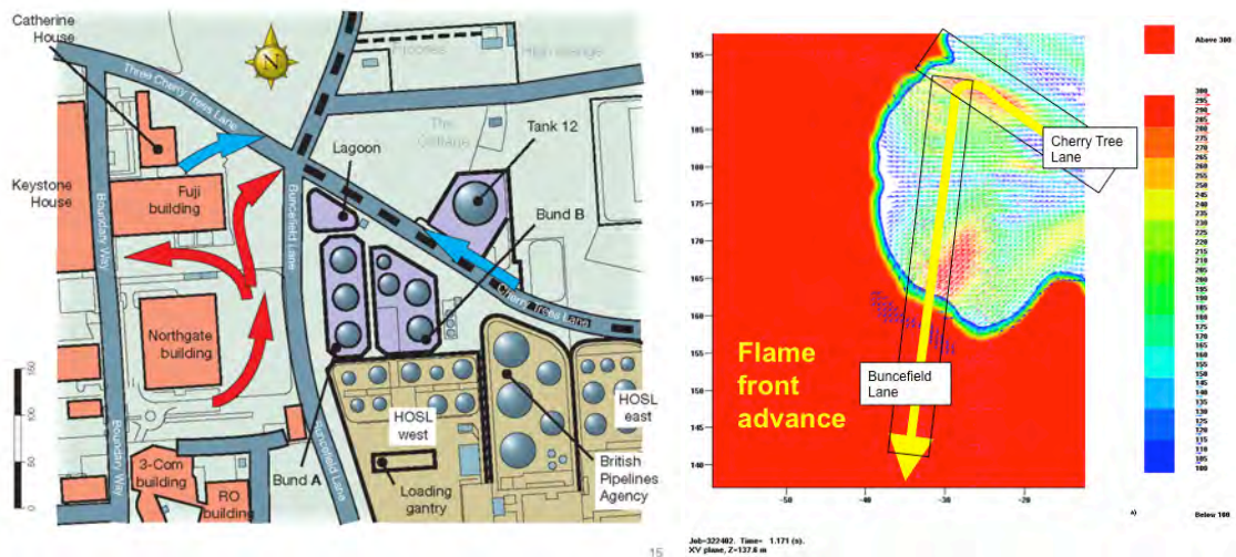
Figure 8: Directional movement of objects (BMIIB final report vol. 2) and predicted flow pattern using FLACS simulations for actual, extremely dense vegetation.
