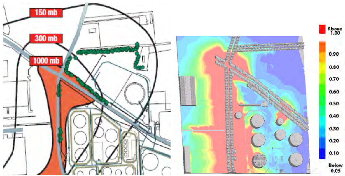
Figure 6: Predicted overpressures (right) compared to estimated pressures in BMIIB final report (left)
