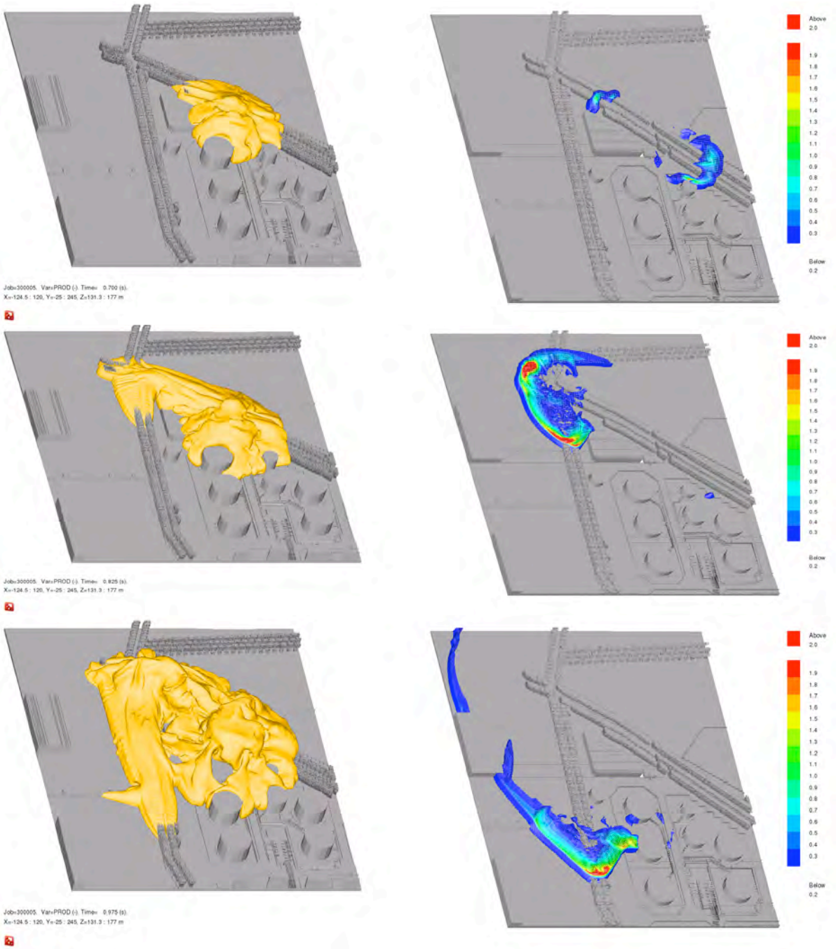
Figure 5: FLACS explosion simulation of the Buncefield depot with extremely dense vegetation. Flame propagation (left) and resulting overpressures in bars (right).
