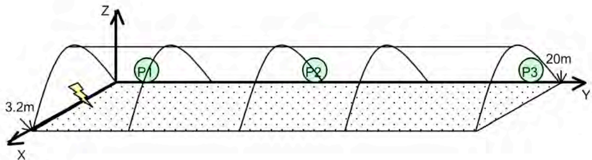
Figure 9: Schematic drawing of the experimental set-up used during this work showing the position of the ignition source and pressure transducers.
