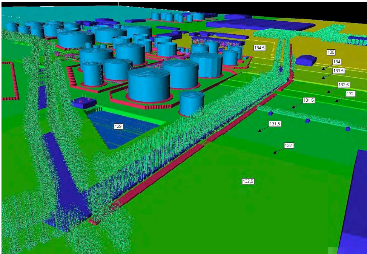
Figure 2 FLACS model of the Buncefield tank farm, looking south
