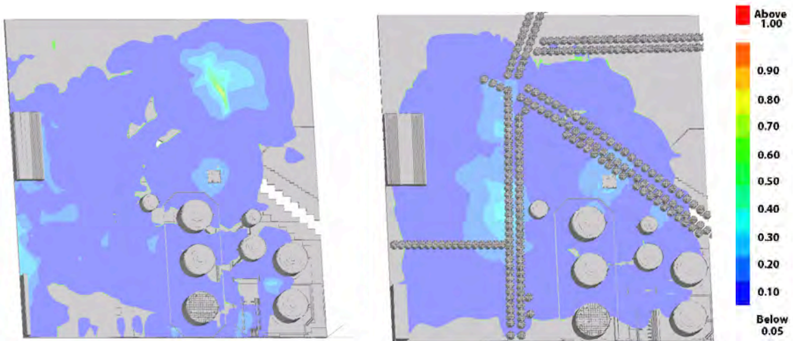
Figure 7: Predicted overpressures with no trees (left) compared to simulations with more traditional trees with large trunks (right).
