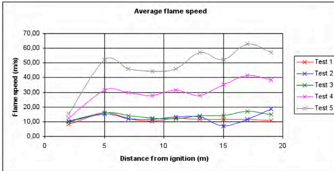
Figure 10: The average flame speed as a function of the distance from the ignition source.
